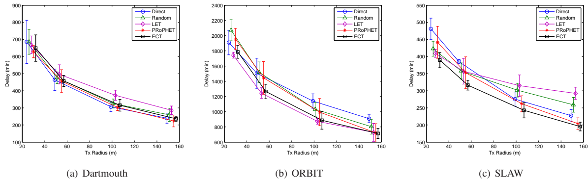
Fig. 10. Average routing delays of various protocols under Dartmouth, ORBIT and SLAW.
