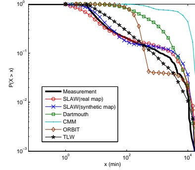
Fig. 7. Flight length distributions of synthetic traces from various models.
